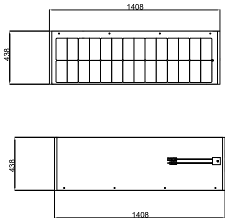
All Dimensions in mm The above drawing is a graphical representation of the product.
