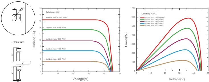
Current-Voltage & Power-Voltage Curves (SKT585M12-120D5)
