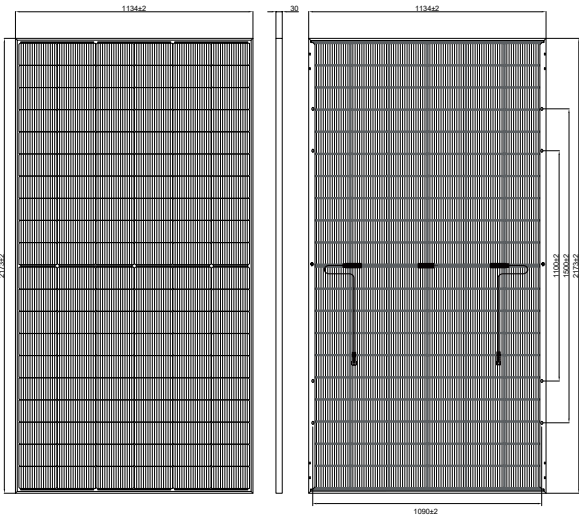
All Dimensions in mm The above drawing is a graphical representation of the product.
