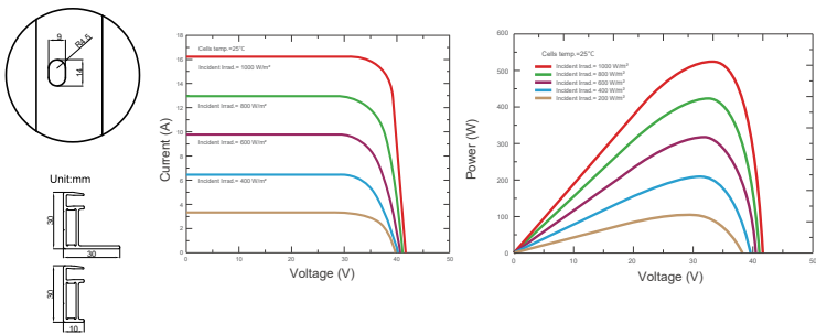
Current-Voltage & Power-Voltage Curves (SKT525M12-108D5)
