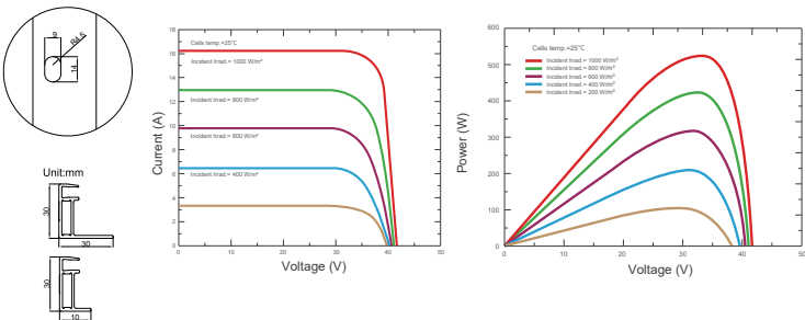
Current-Voltage & Power-Voltage Curves (SKT525M12-108D4)
