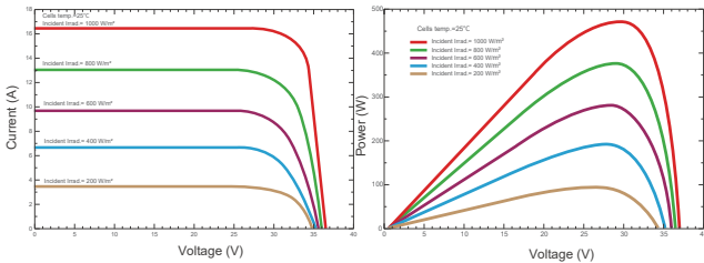
Current-Voltage & Power-Voltage Curves (SKT470M12-96D4)
