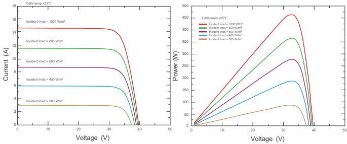
Current-Voltage & Power-Voltage Curves (SKT460M10-108D4)
