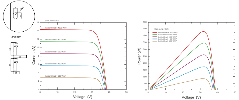
Current-Voltage & Power-Voltage Curves (SKT430M10-108D4)
