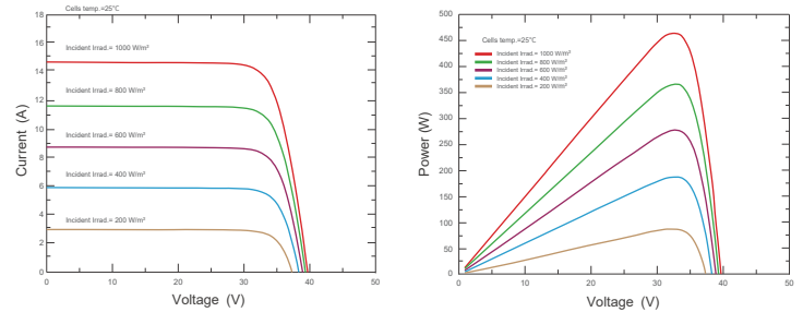
Current-Voltage & Power-Voltage Curves (SKT460M10-108D6)
