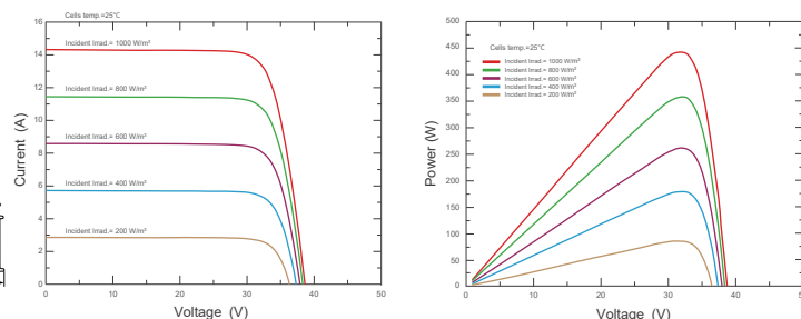
Current-Voltage &amp; Power-Voltage Curves (SKT440M10-108D4)
