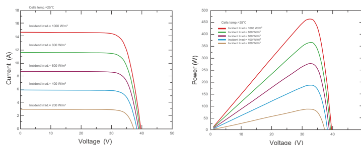
Current-Voltage & Power-Voltage Curves (SKT460M10-108D5)
